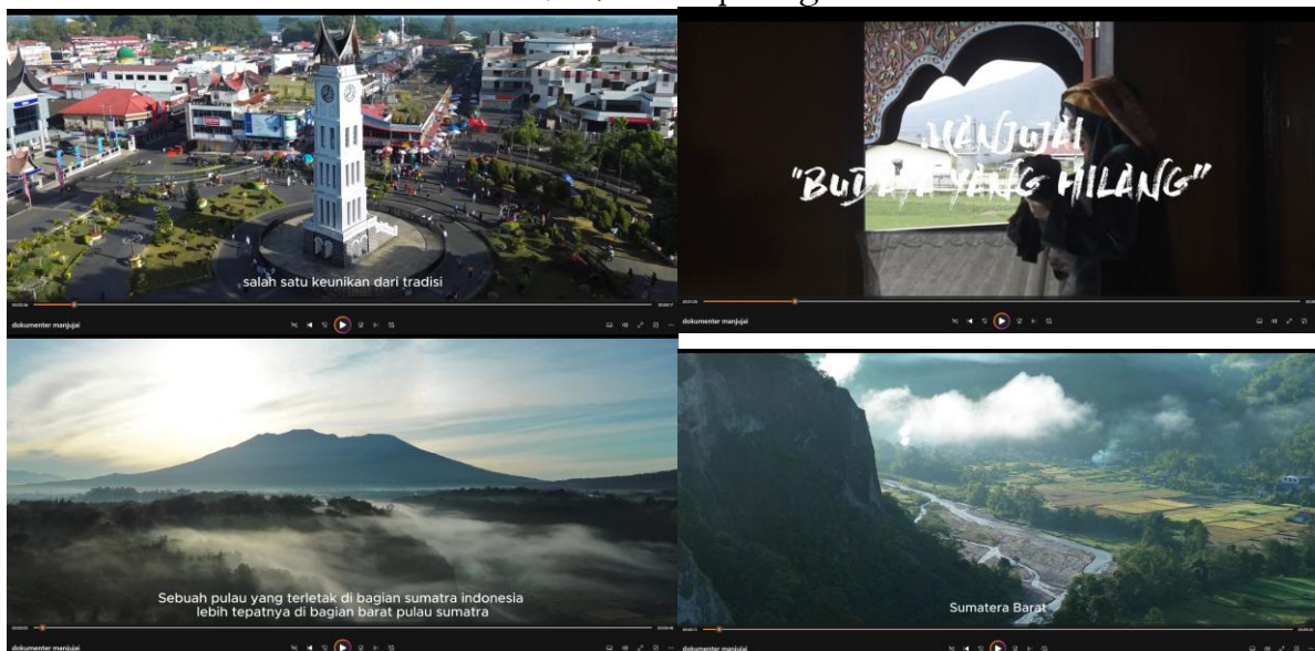
Gambar 5. Opening Scene
