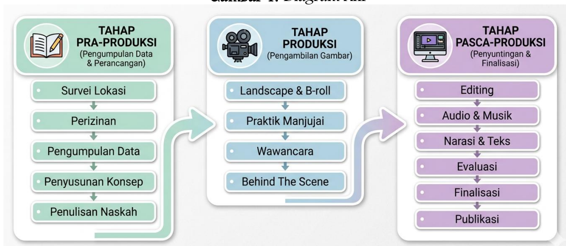
Gambar 1. Diagram Alir
